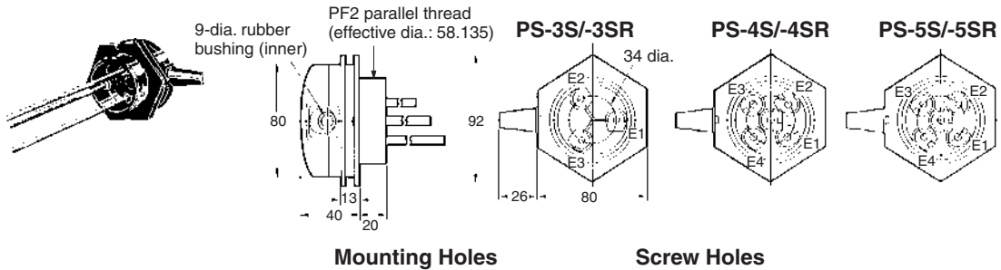
Mounting Holes
